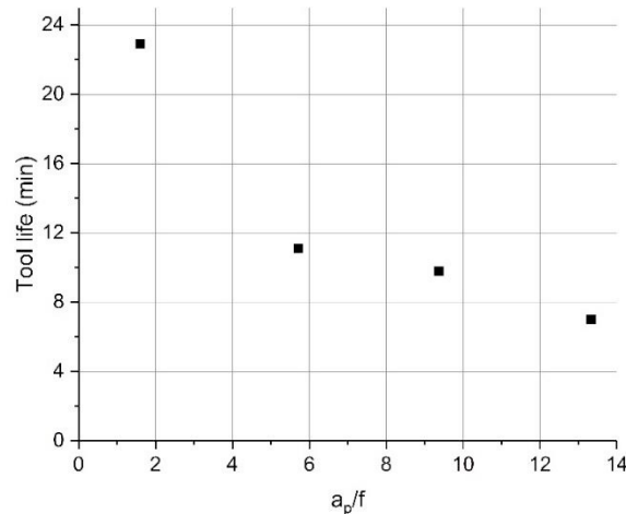
Fig. 2. The tool life as a function of a_p/f for case 2, h_e = 0.26 mm.
